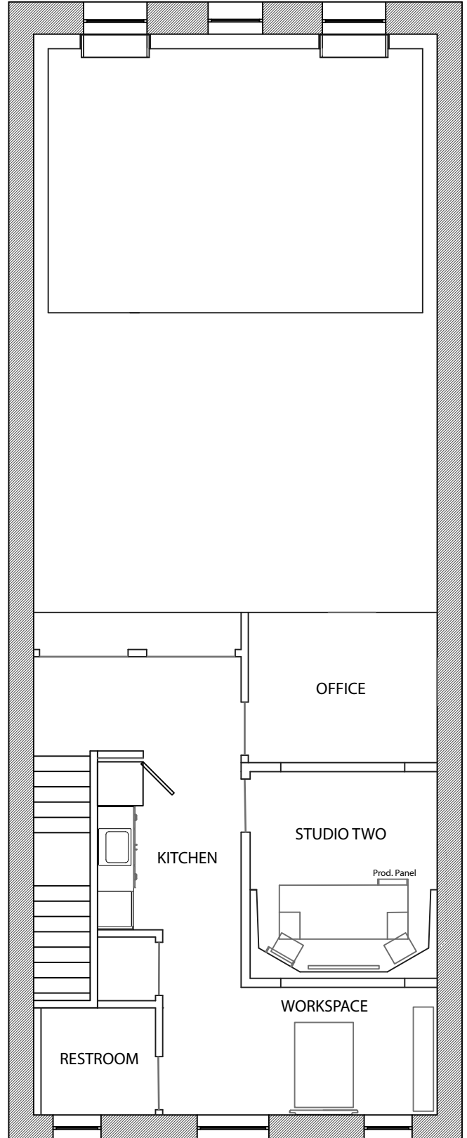
B MEZZANINE PLAN
